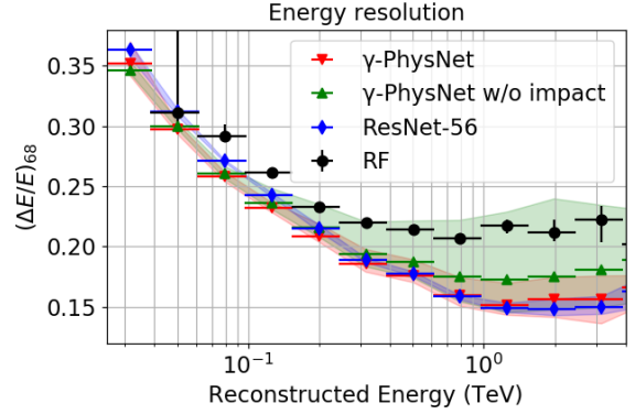
Figure 4: Energy resolution as a function of the energy in the LST energy range (lower is better). Comparison of the performance on the energy regression task between the probed models.
